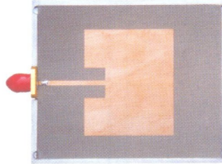
II. Rectangular Microstrip Patch Antenna with Inset feed
